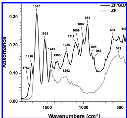
Figure 2. IR spectra of zein film (ZF) and film from zein cross-linked with 16% (wt/wt % based on protein) glutaraldehyde (ZF/GDA).
